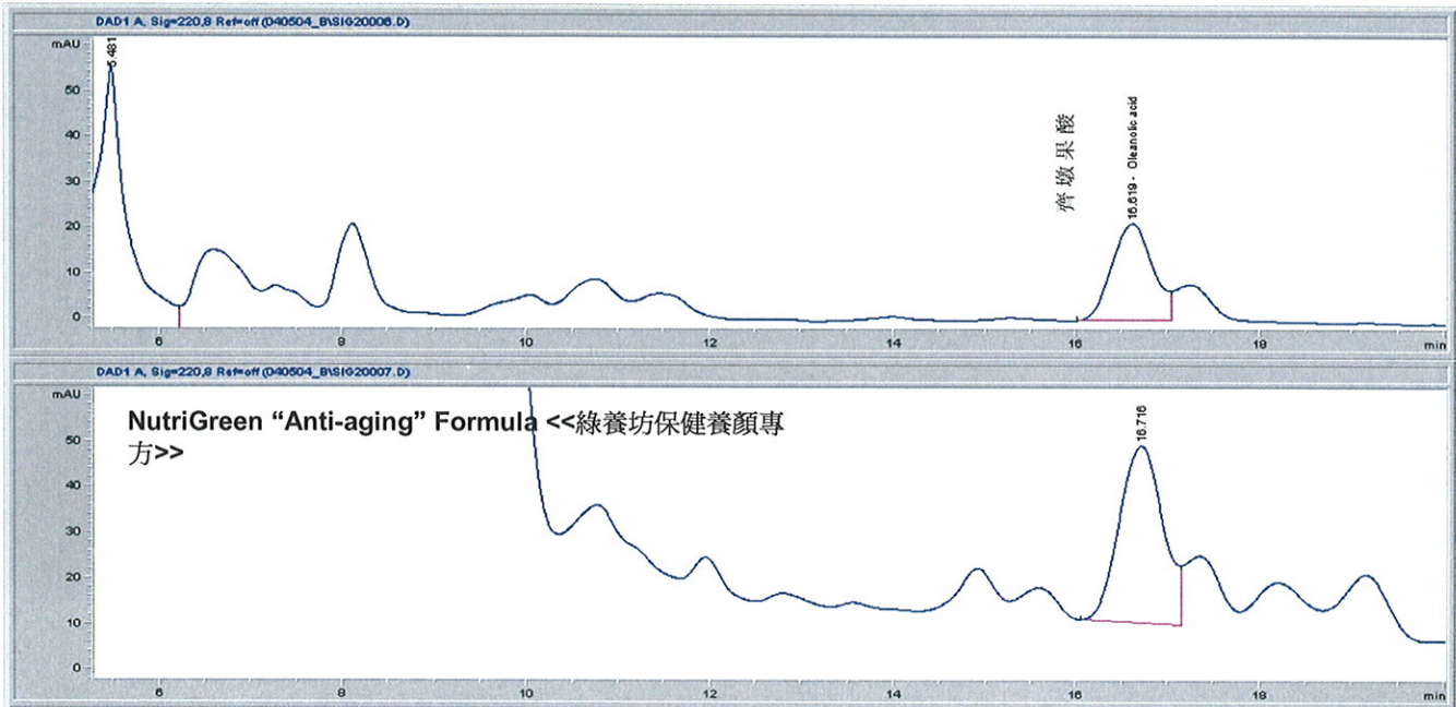
Figure 3. High Performance Liquid Chromatography (HPLC) Fingerprint Analysis of Fructus Ligustri Lucidi and NutriGreen “Anti-aging” Formula.
